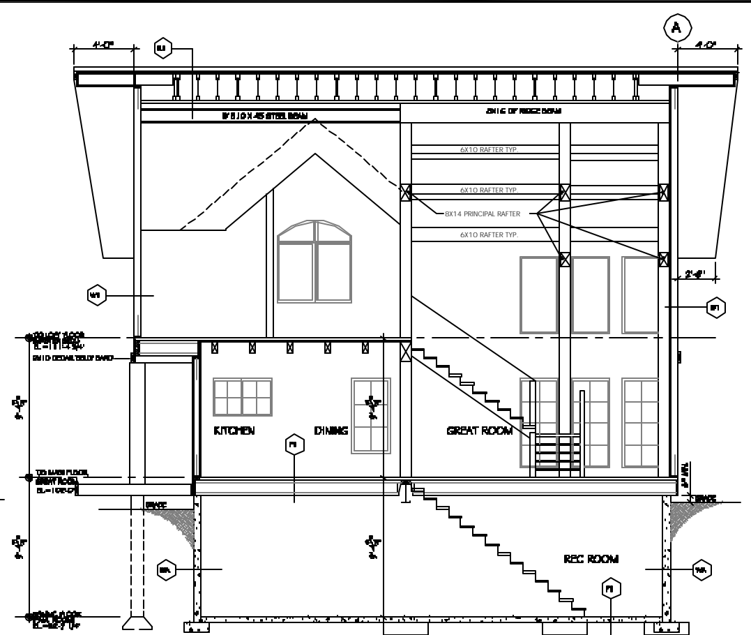
B-B BUILDING SECTION SCALE 1/4" = 1'-0"
