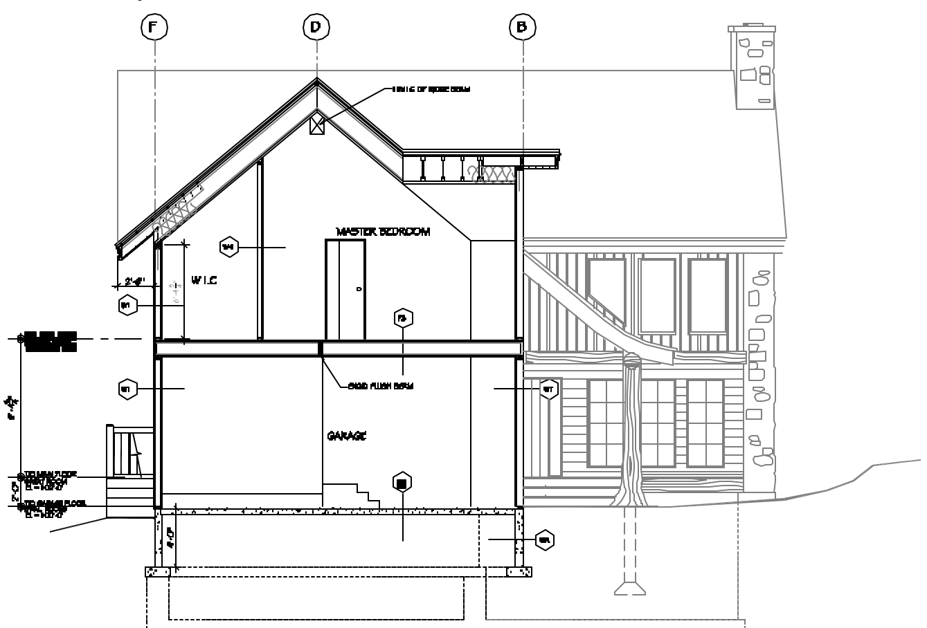
C-C BUILDING SECTION SCALE 1/4" = 1'-0"
