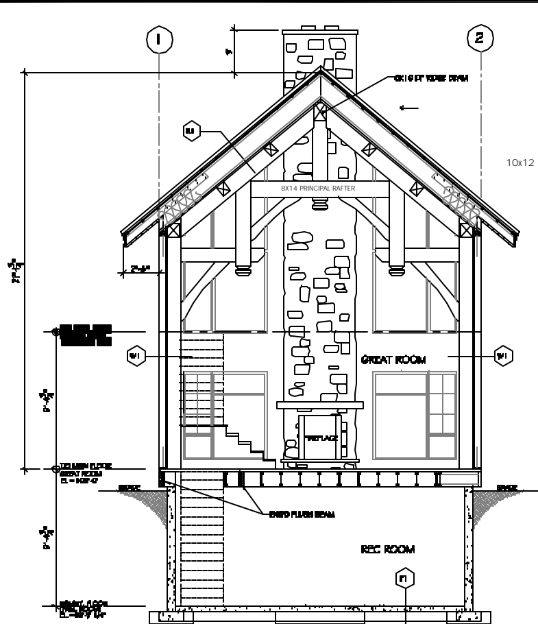
A-A BUILDING SECTION SCALE 1/4" = 1'-0"
