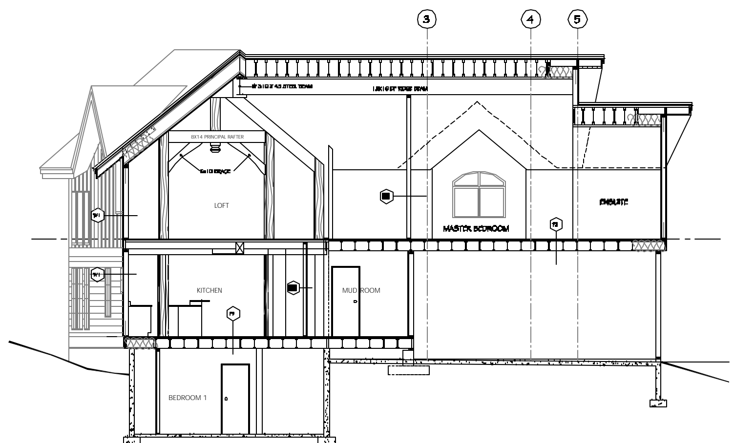
D-D BUILDING SECTION SCALE 1/4" = 1'-0"
